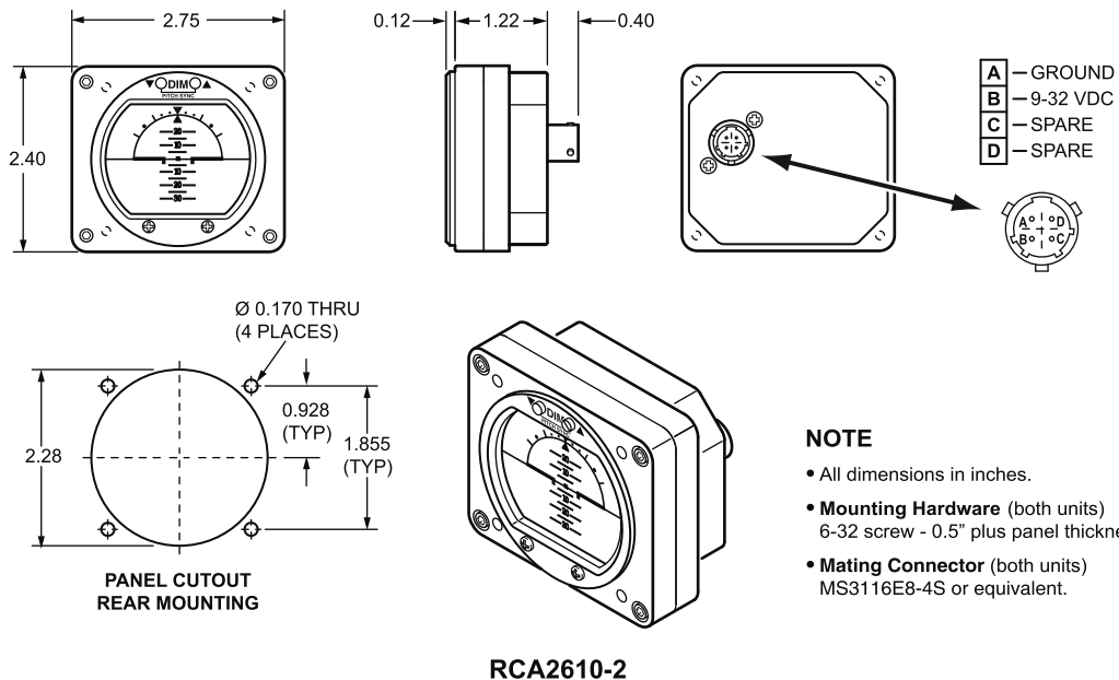
Figure 1.1, General Dimensions
