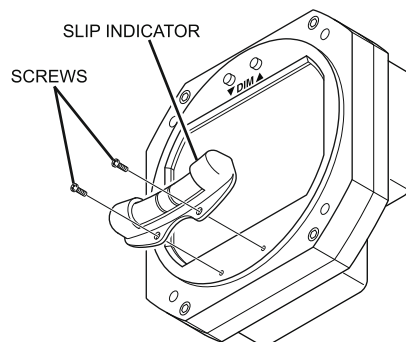
Figure 4.1, Inclinometer Installation
