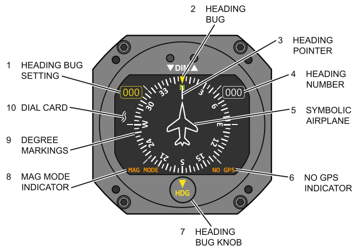
Figure 1.2, Typical Display Features
