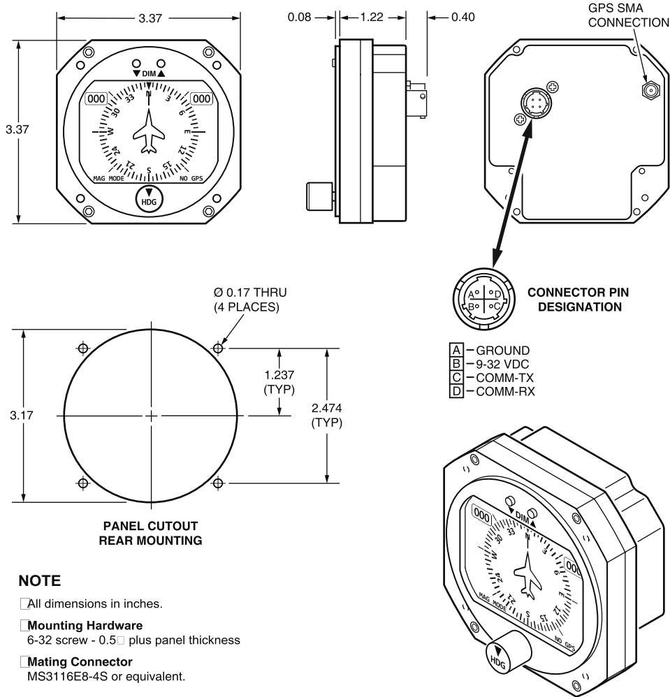
Figure 1.1, General Dimensions
