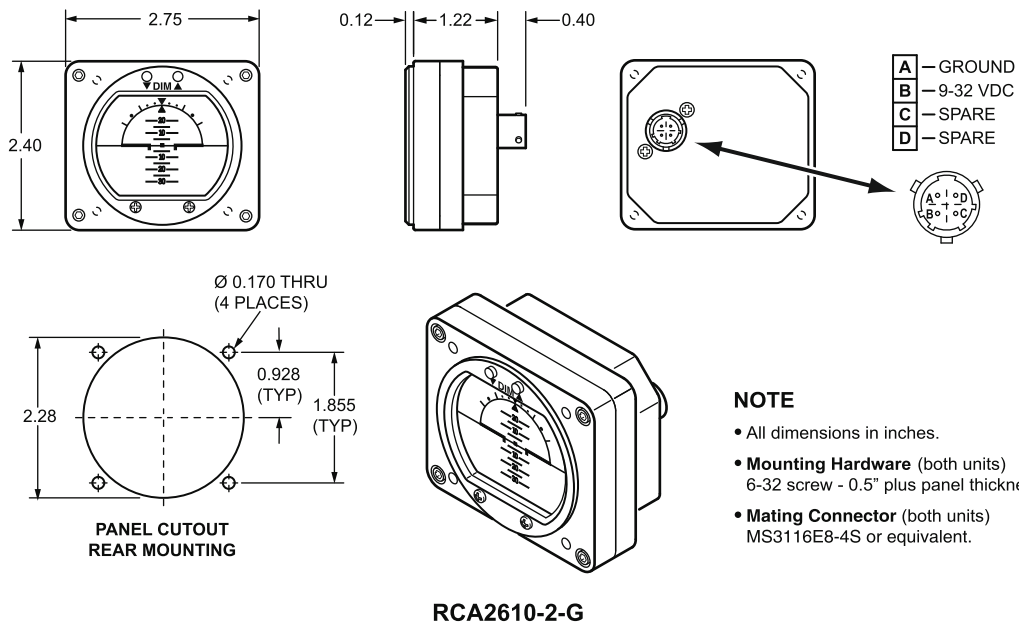
Figure 1.2, General Dimensions (-G Models)
