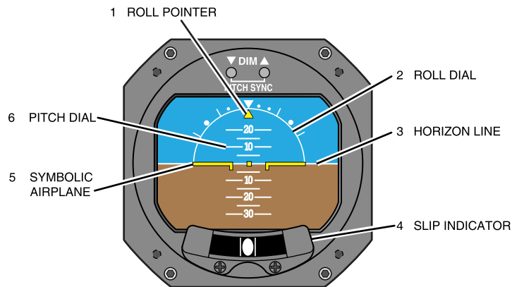
Figure 1.3, Typical Display Features
