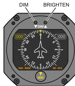
Figure 3.2, Dimmer Controls
